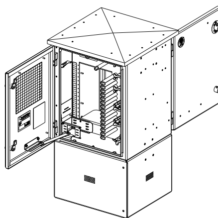
144 with 12" (304.80 mm) Riser
