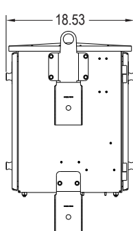
144 with Pole Mount Kit - Dimensions
