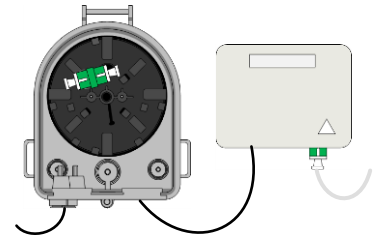
YOURx-TAP and CraftSmart Fiber Outlet
