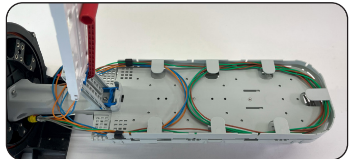
Example of use for fiber slack storage Intermittently Bonded Ribbon (IBR).
