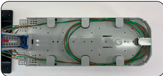
Example of use for ribbon fiber slack storage using transfer tubes.
