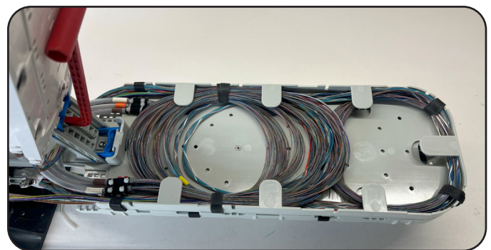
Example of use for fiber slack storage Intermittently Bonded Ribbon (IBR).
