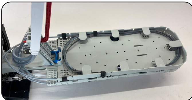
Example of use for ribbon fiber slack storage using transfer tubes.
