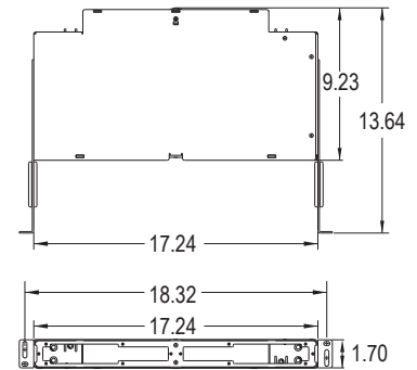
Rack Mount SCD Panel with xPAK and Clearview Blue Cassette
