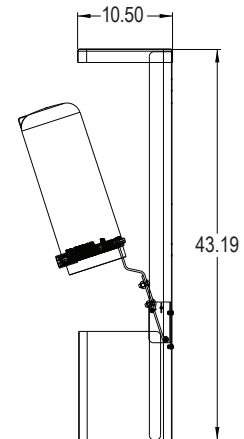
Tilting Pedestal Bracket 014304
